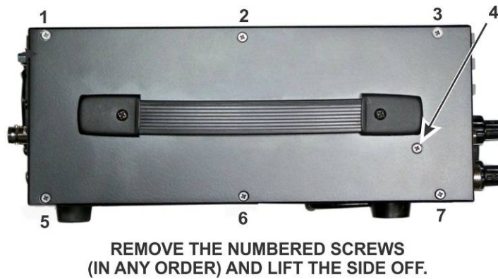
Figure 96. Removing the Left Side Panel.
