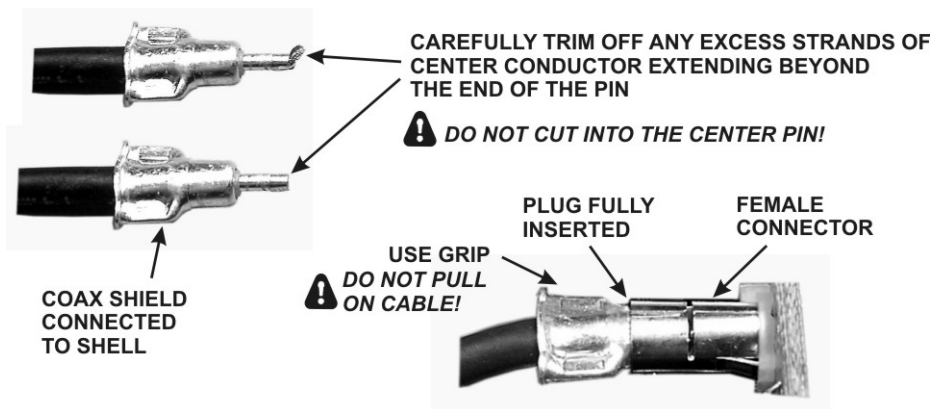
Figure 81. TMP Cable Connectors.
