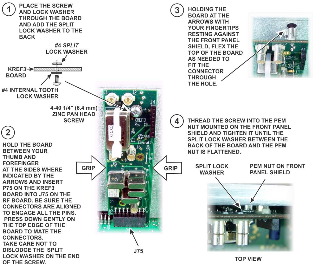
Figure 78. Installing KREF3 Board.
