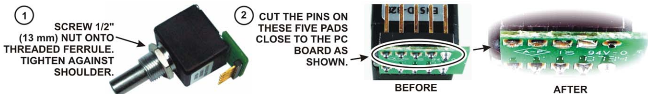
Figure 14. VFO B Encoder Assembly Preparation for Installation.
