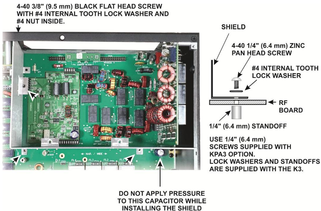
Figure 87. Attaching the KPA3A Shield.
